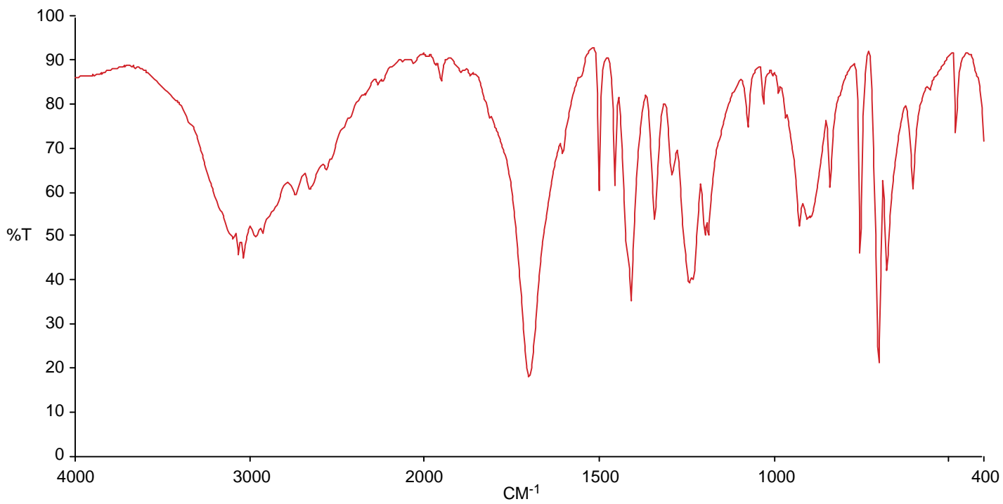
Figure 3 Correctly Prepared KBr Disk of Phenyl Acetic Acid
